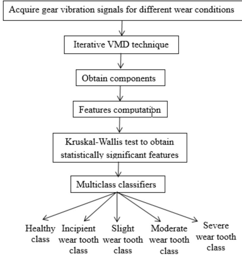
Figure 3. 2 Procedure of the proposed method
