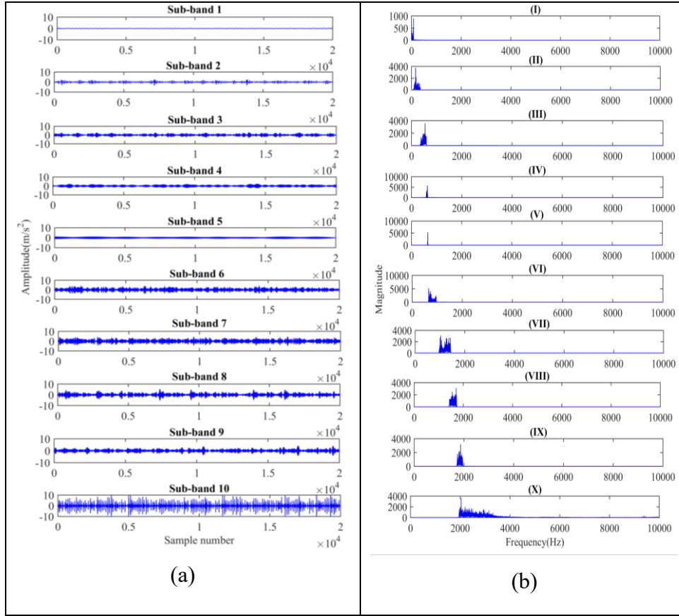
Figure 4. 5 (a) Applied EWT decomposition and find sub-bands, (b) Represent the magnitude spectrum of their respective sub-bands.
