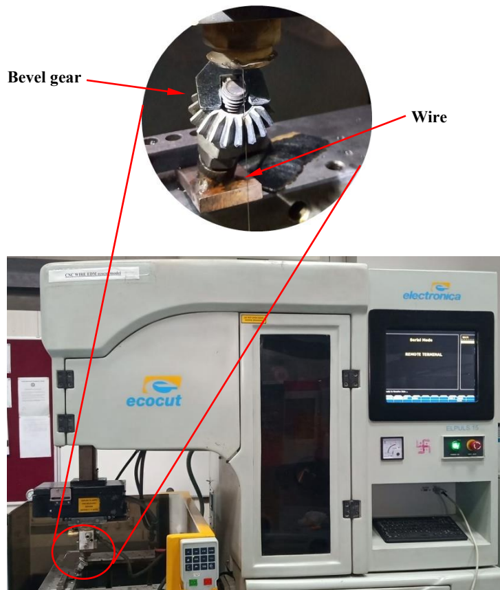
Figure 4. 3 Crack faults created by CNC wire (EDM) machine.
