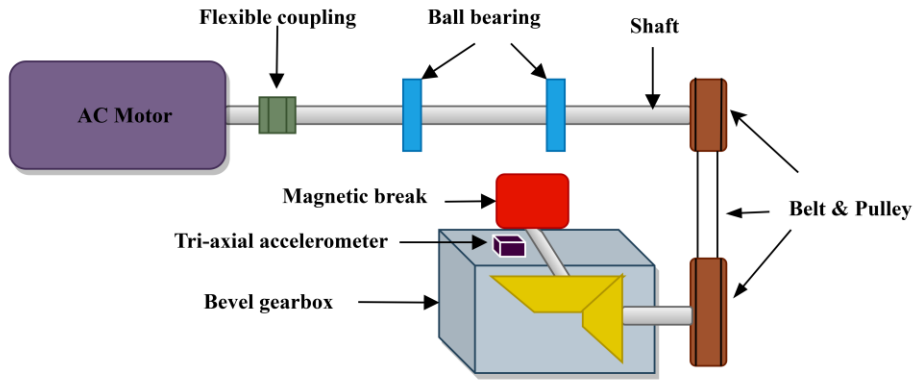
Figure 2. 3 The schematic representation of the MFS.
