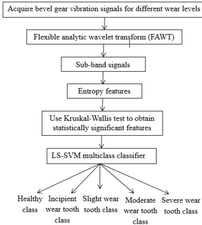
Figure 2. 1 Block diagram of the proposed method
