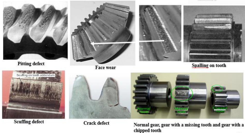
Figure 1. 2 Various type of gear faults. [Ref: Google images]
