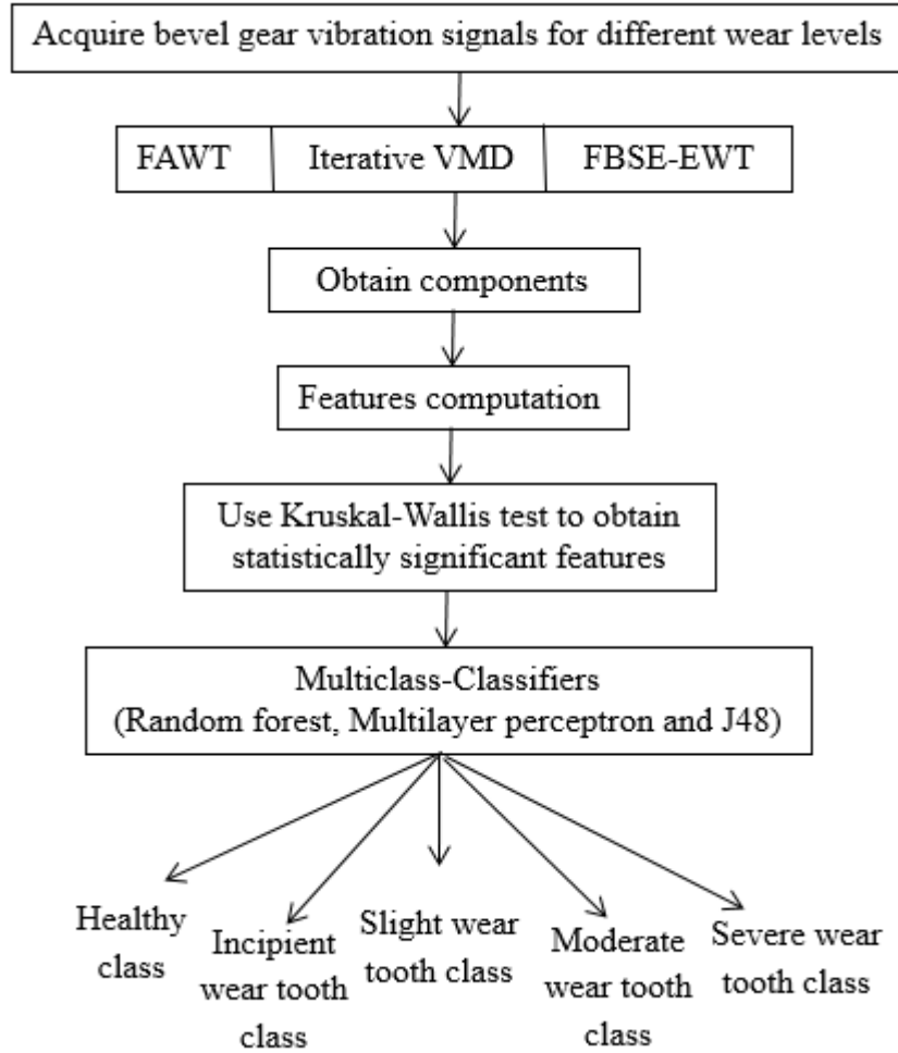
Figure 5. 1 A block diagrammatic representation of the methodology
