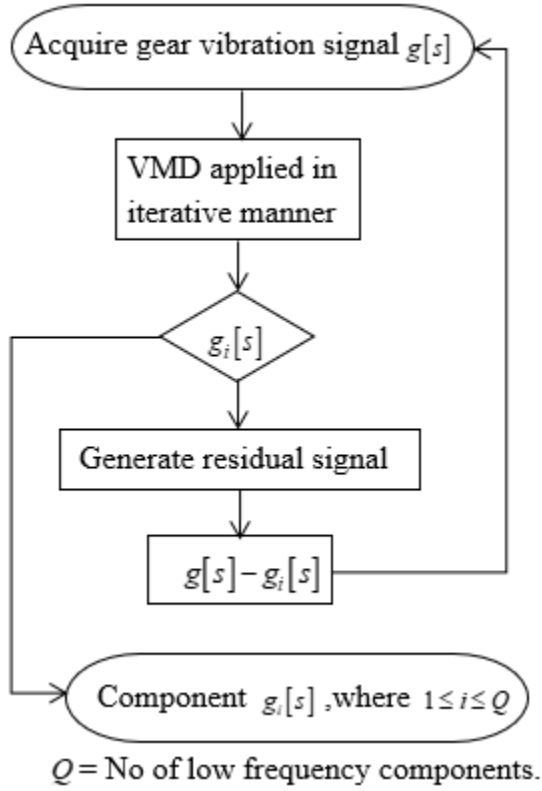
Figure 3. 3 Flowchart of proposed iterative VMD technique
