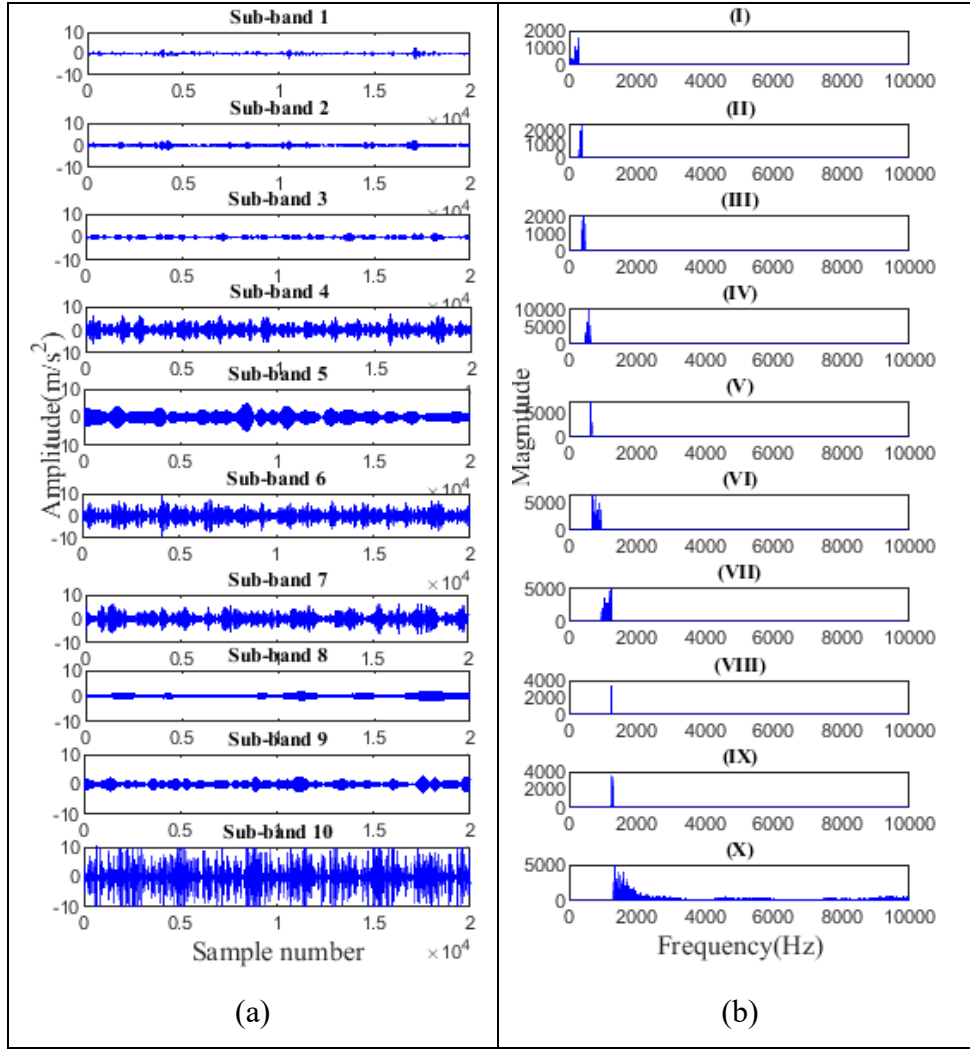
Figure 5. 4 (a) Applied FBSE-EWT decomposition and find sub-bands, (b) Represent the magnitude spectrum of their respective sub-bands.
