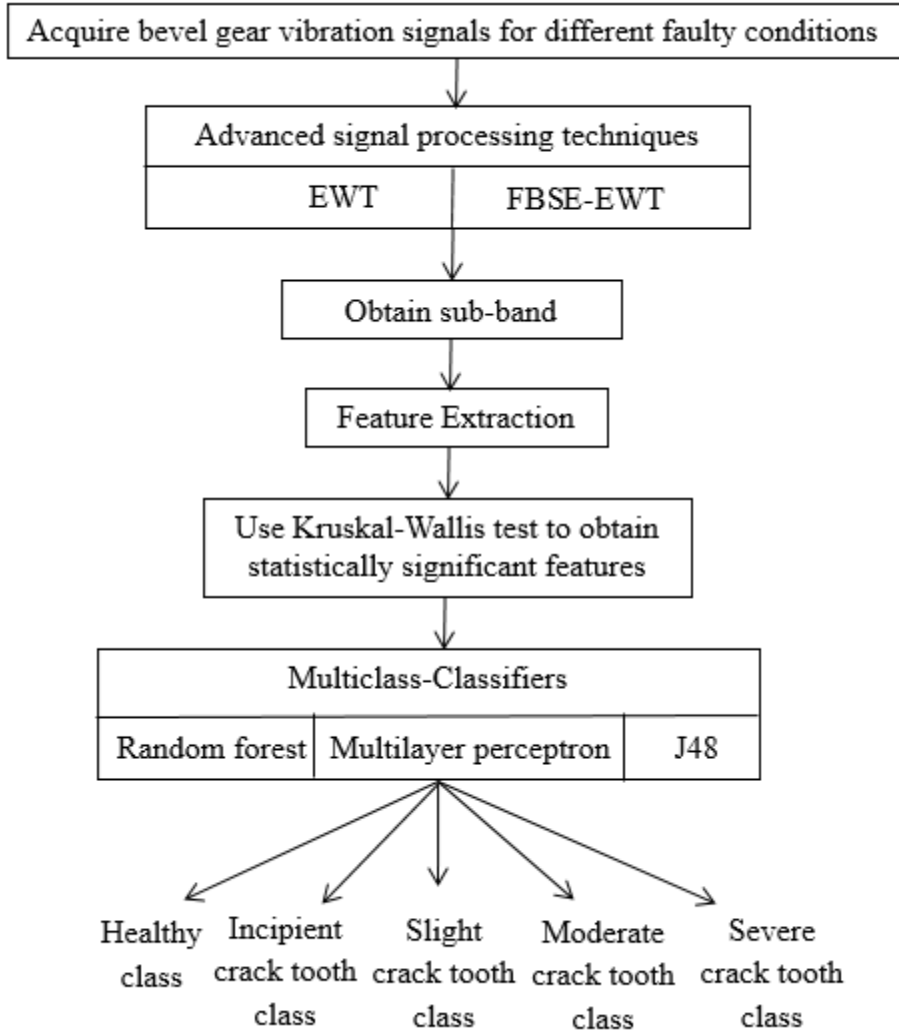
Figure 4. 1 Block diagram showing the suggested approach.
