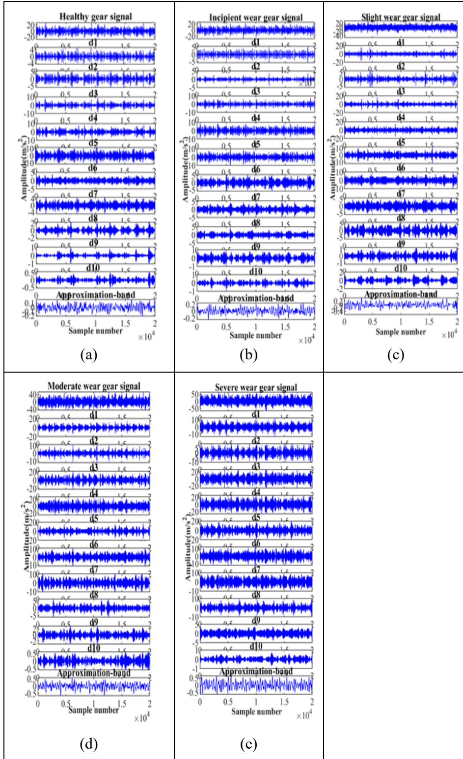
Figure 2. 6 Applied FAWT decomposition (10 levels) on gear signals. (a) healthy gear signal, (b) incipient wear gear signal, (c) slight wear gear signal, (d) moderate wear gear signal, (e) severe wear gear signal
