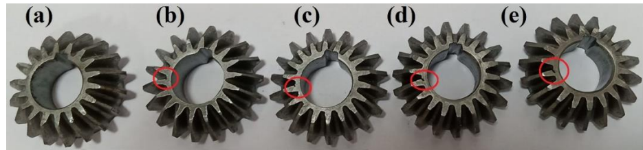
Figure 4. 4 Health of the gears (a) Healthy gear (b) Gear with 0.25 mm crack length (c) Gear with 0.50 mm crack length (d) Gear with 0.75 mm crack length (e) Gear with 1.00 mm crack length
