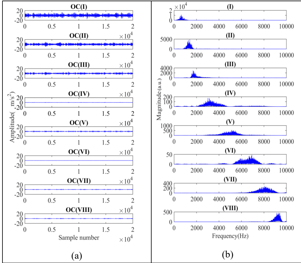
Figure 3. 4 (a) Plots of the OCs using iterative VMD method for healthy bevel gear signal, (b) Plots of the magnitude spectrum of respective OCs using iterative VMD method for healthy bevel gear signal. The unit of Y axis are arbitrary.
