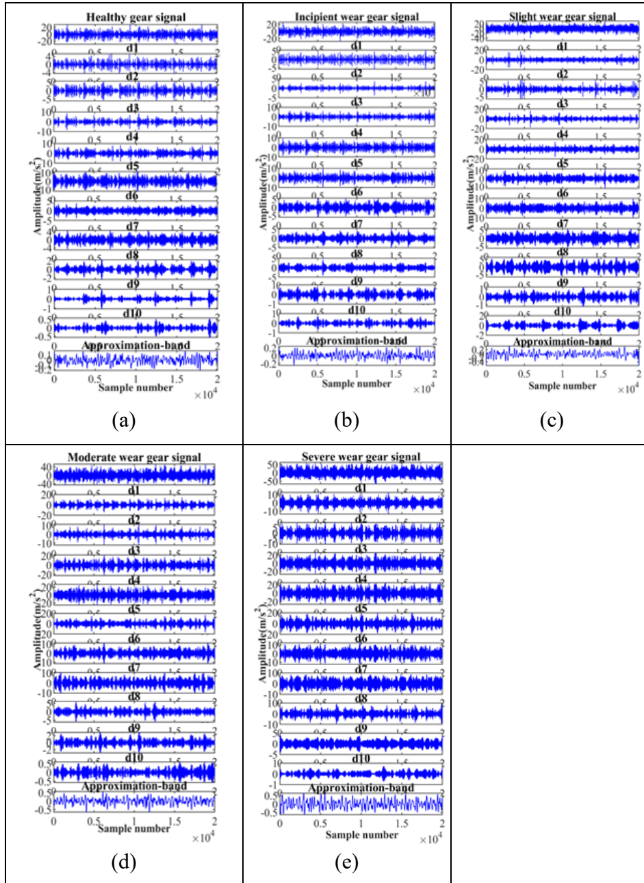
Figure 5. 2 Applied FAWT decomposition (10 levels) on gear signals. (a) healthy gear signal, (b) incipient wear gear signal, (c) slight wear gear signal, (d) moderate wear gear signal, (e) severe wear gear signal
