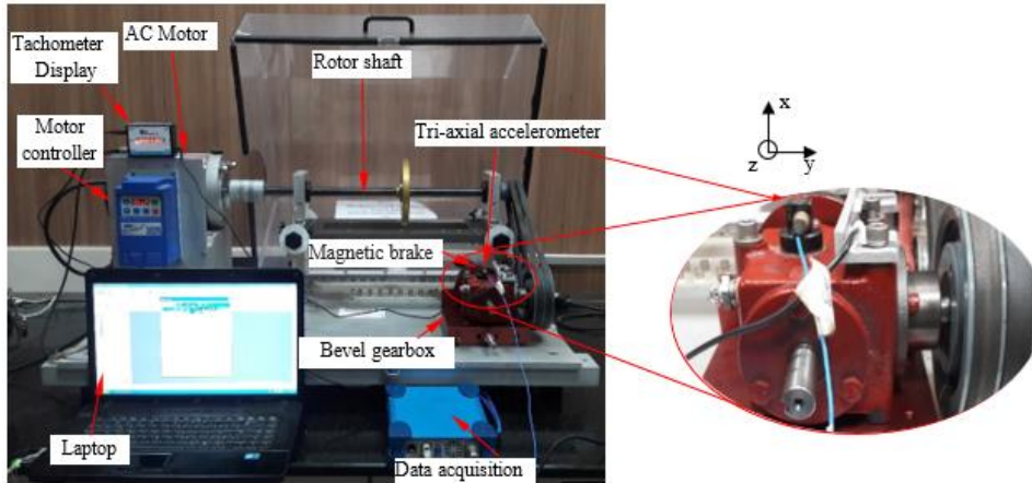
Figure 2. 2 Experimental test setup with the zoomed view of the accelerometer.
