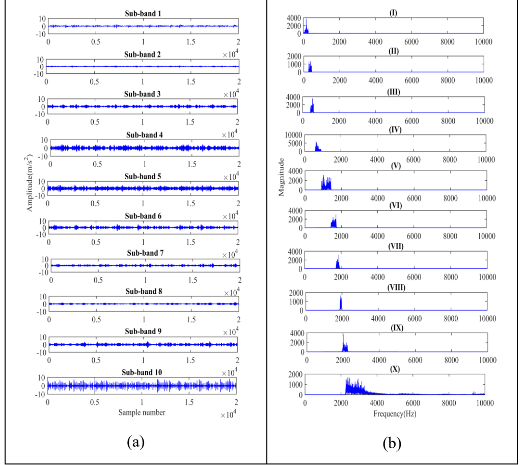
Figure 4. 6 (a) Applied FBSE-EWT decomposition and find sub-bands, (b) Represent the magnitude spectrum of their respective sub-bands.
