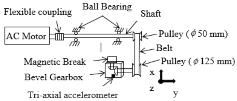
Figure 4. 2 The schematic presentation of the experimental setup.
