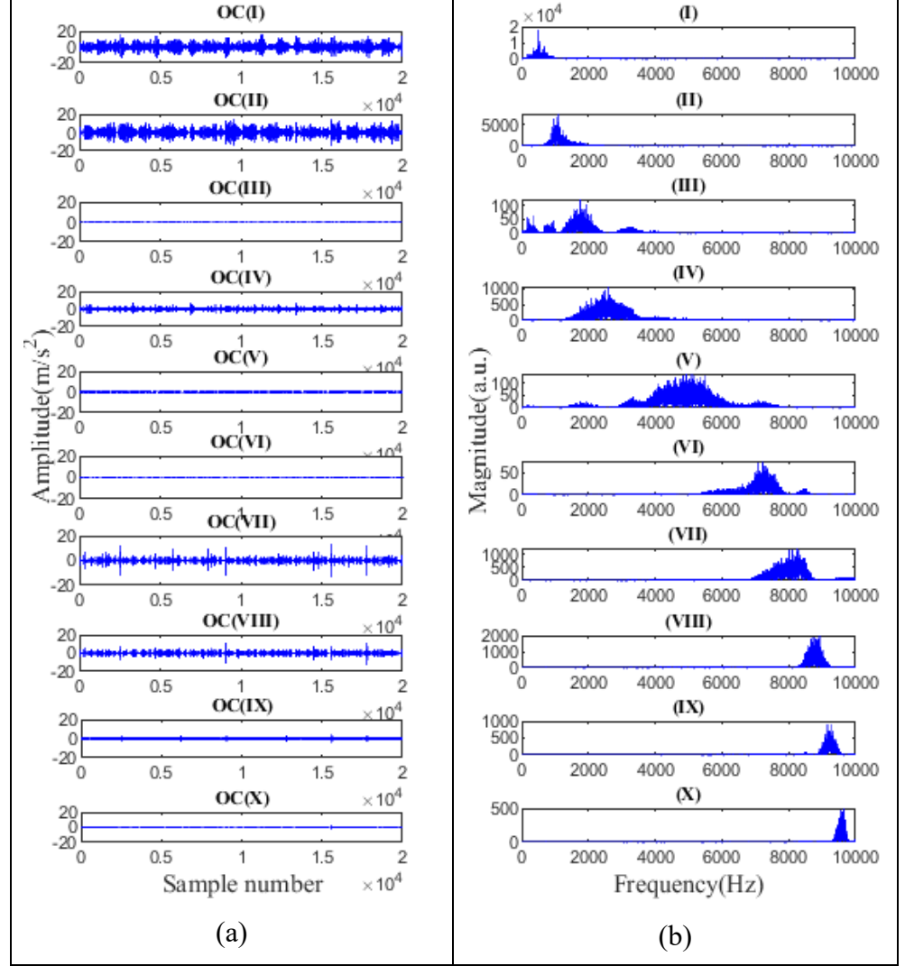
Figure 5.3 (a) Plots of the OCs using method for healthy bevel gear signal. (b) Plots of the magnitude spectrum of respective OCs using iterative VMD method for healthy bevel gear signal. The unit of Y axis are arbitrary.
